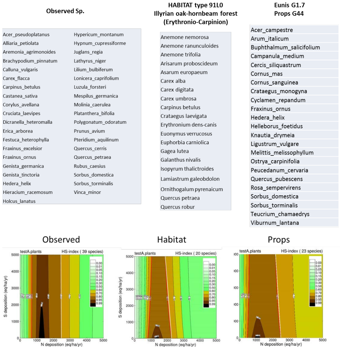
Figure IT-2. Site IT07.
