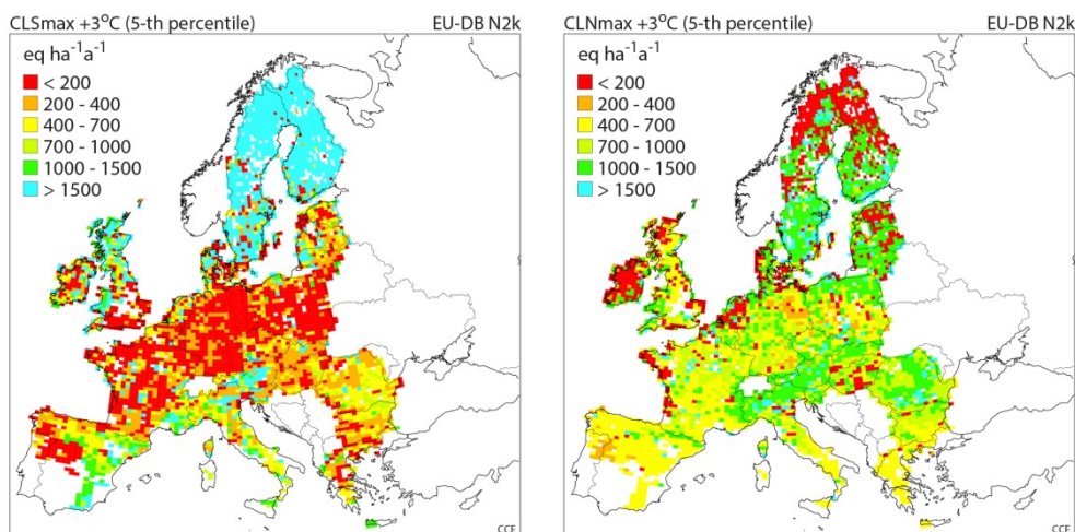
Figure 1.13 Natura 2000 critical loads of biodiversity using the European background database for sulphur (left) and for nitrogen (right) under a +3^{\circ}\text{C} increase of the annual mean surface air temperature
