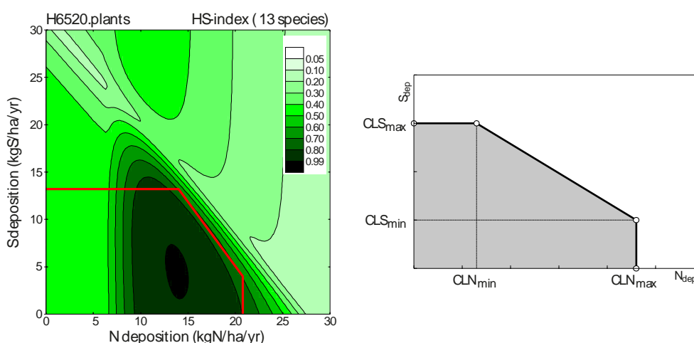
Figure 1.4 Left: A nitrogen-sulphur critical load function (N-S CLF) for biodiversity derived from the chosen HS index limit value (80% of maximum; red line). Right: The N-S CLF defined by the maximum and minimum critical loads of biodiversity for sulphur ( CLS_{max} and CLS_{min} ) and for nitrogen ( CLN_{min} and CLN_{max} ) (Source: Posch et al. 2015a)
