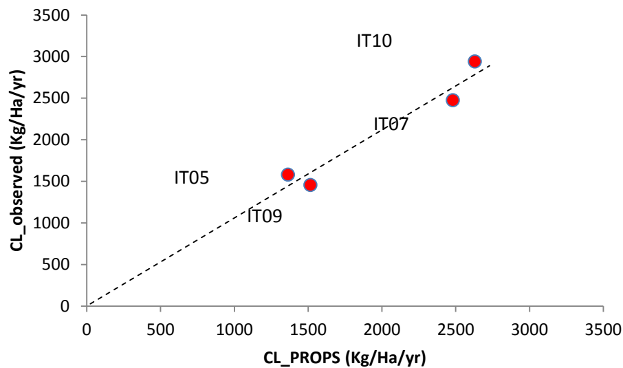
Figure IT-6. Critical loads based on observed plant lists living in the test sites are closely similar to Critical loads predicted by PROPS that, pointing thus a high naturalness of these sites being also able to tolerate actual N deposition.
