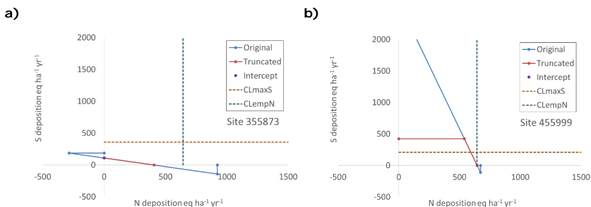
Figure UK-2. Examples of sites where the values originally fitted for CL_{Smax} , CL_{Smin} , CL_{Nmax} and/or CL_{Nmin} were outside a reasonable range, which we defined as between zero and 2 \times CL_{maxS} for S, or between zero and 2 \times CL_{empN} for N. Where the original function lay within these ranges, its shape was retained. Values less than zero were increased to zero, as in example a). Where original values were greater than 2 \times CL_{maxS} for S, or greater than 2 \times CL_{empN} for N, they were decreased to these maximum reasonable values, as shown for CL_{Smax} in example b). The UK data submission consisted of these truncated values.
