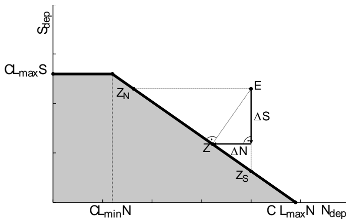
Figure 1.3 Critical load function (CLF) of acidifying nitrogen and sulphur in the (N_{dep}, S_{dep}) plane of computed nitrogen and sulphur deposition. The grey area denotes pairs for which there is non-exceedance. The critical load exceedance from point E is computed as \Delta S + \Delta N (Source: Fig. 6.5 in Posch et al. , 2015b)
